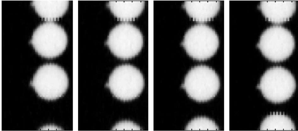
Fig. 4. Time-resolved X-ray absorption images of a pendulum.
