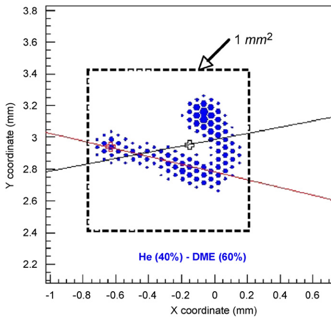
Fig. 5. 6 keV photoelectron track recorded with the X-ray polarimeter.
