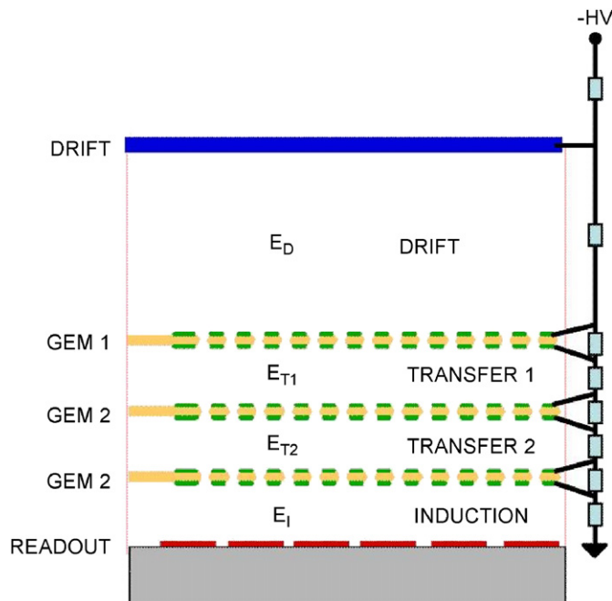
Fig. 1. Schematics of a Triple-GEM detector.
