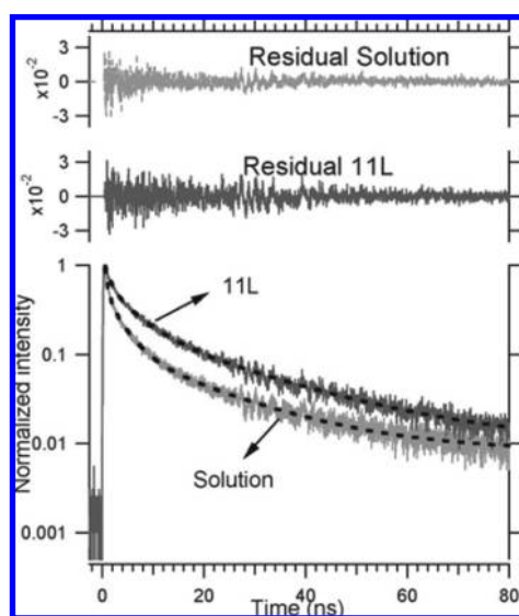
Figure 3. Fluorescence decay profiles of CdSe in solution and in (pLys/CdSe) 11 . The dashed lines show the best fit obtained by eq 1. The curves in the upper panels represent the plots of the weighted residuals for three-exponential fittings.
