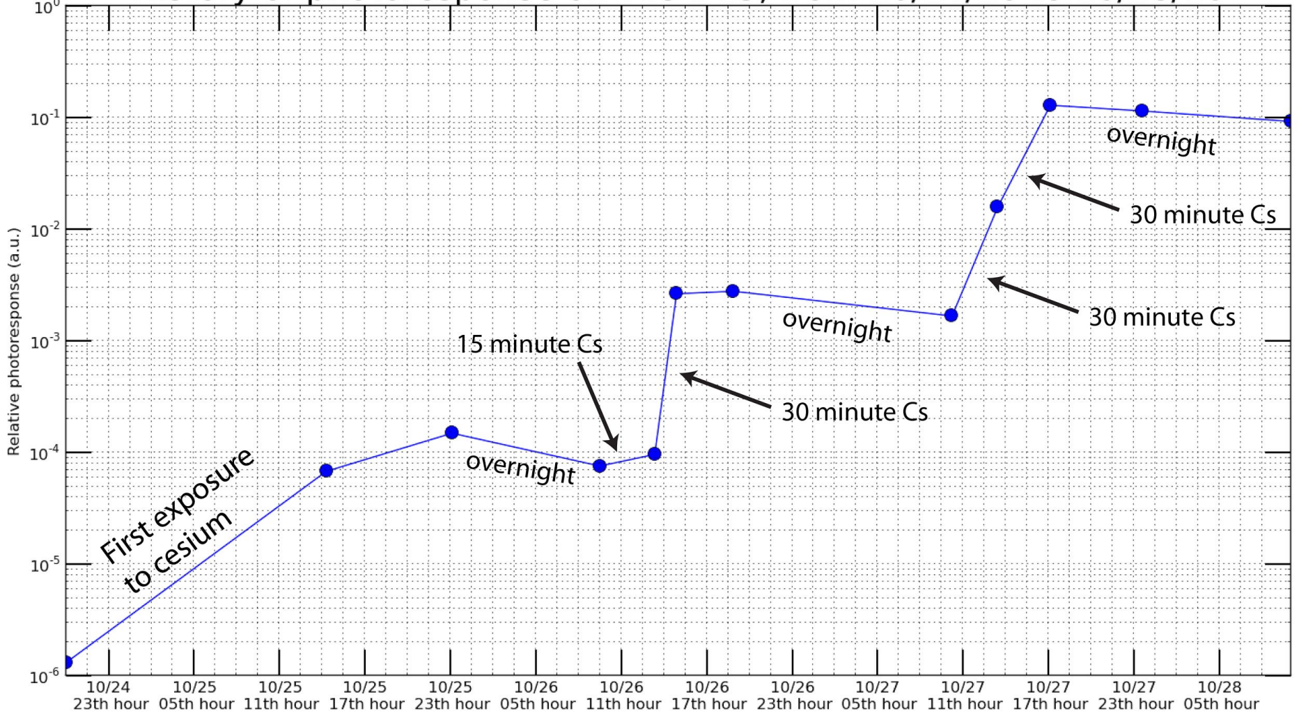
History of photoresponse on Tile #13, from 10/24/16 to 10/28/16
