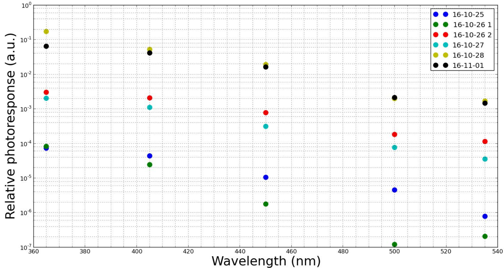
Relative photoresponse vs wavelength over time
